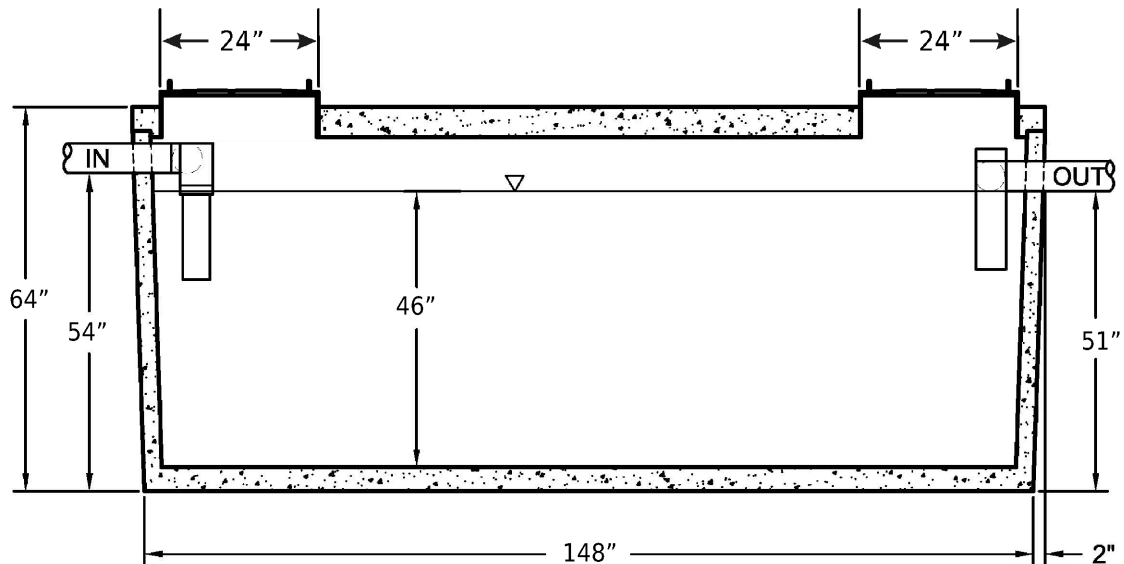
SECTION VIEW
