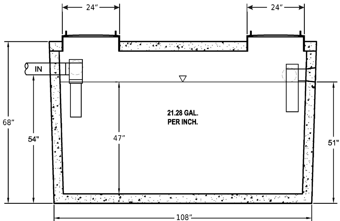
SECTION VIEW
