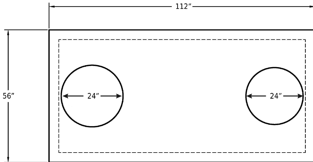
PLAN VIEW
